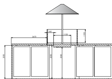
Cross Section
